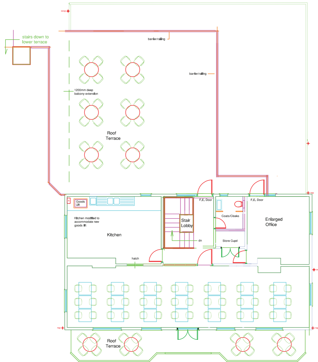
GOLF CLUBHOUSE FIRST FLOOR CONCEPT DESIGN
