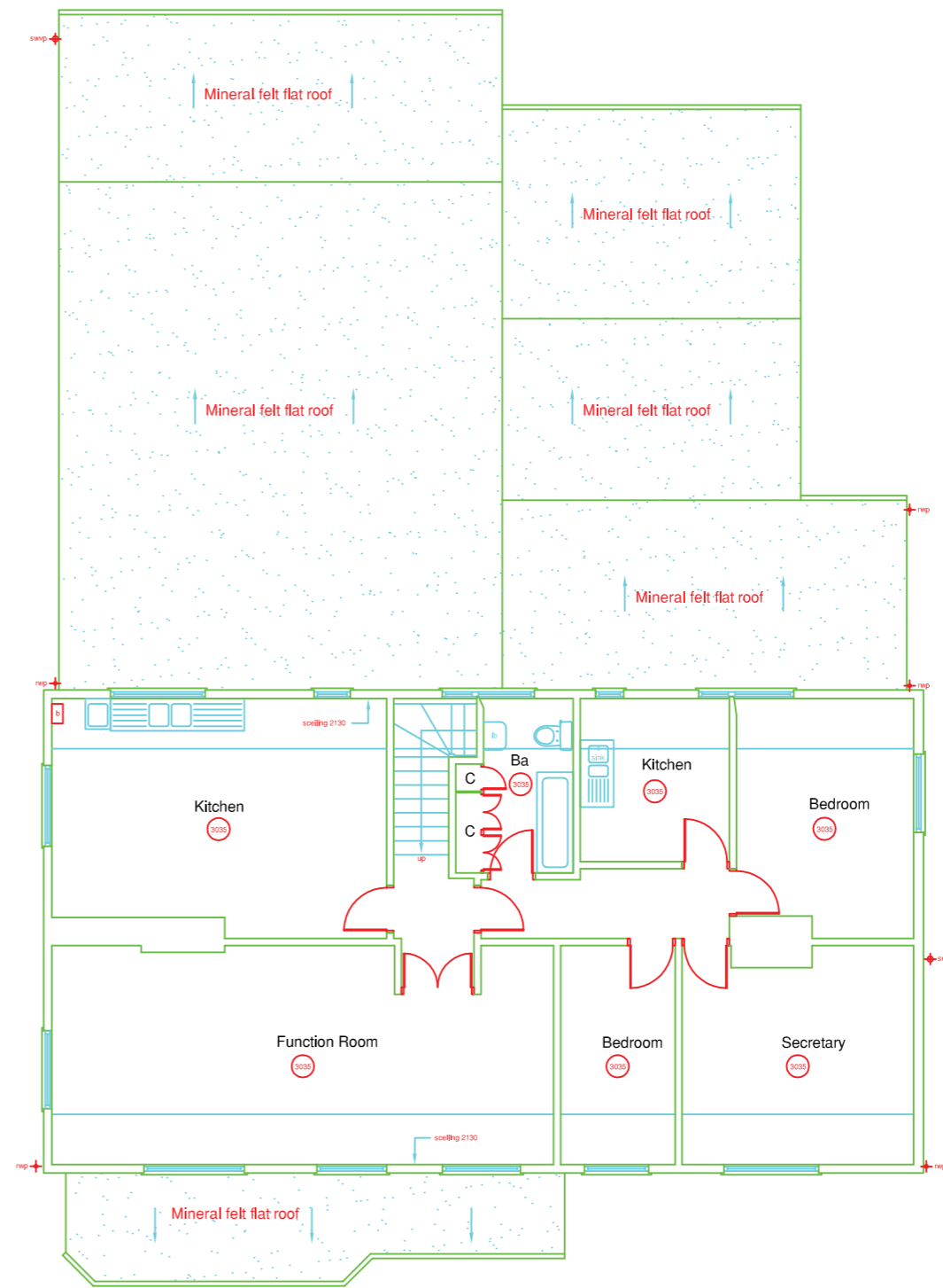
GOLF CLUBHOUSE FIRST FLOOR EXISTING LAYOUT
