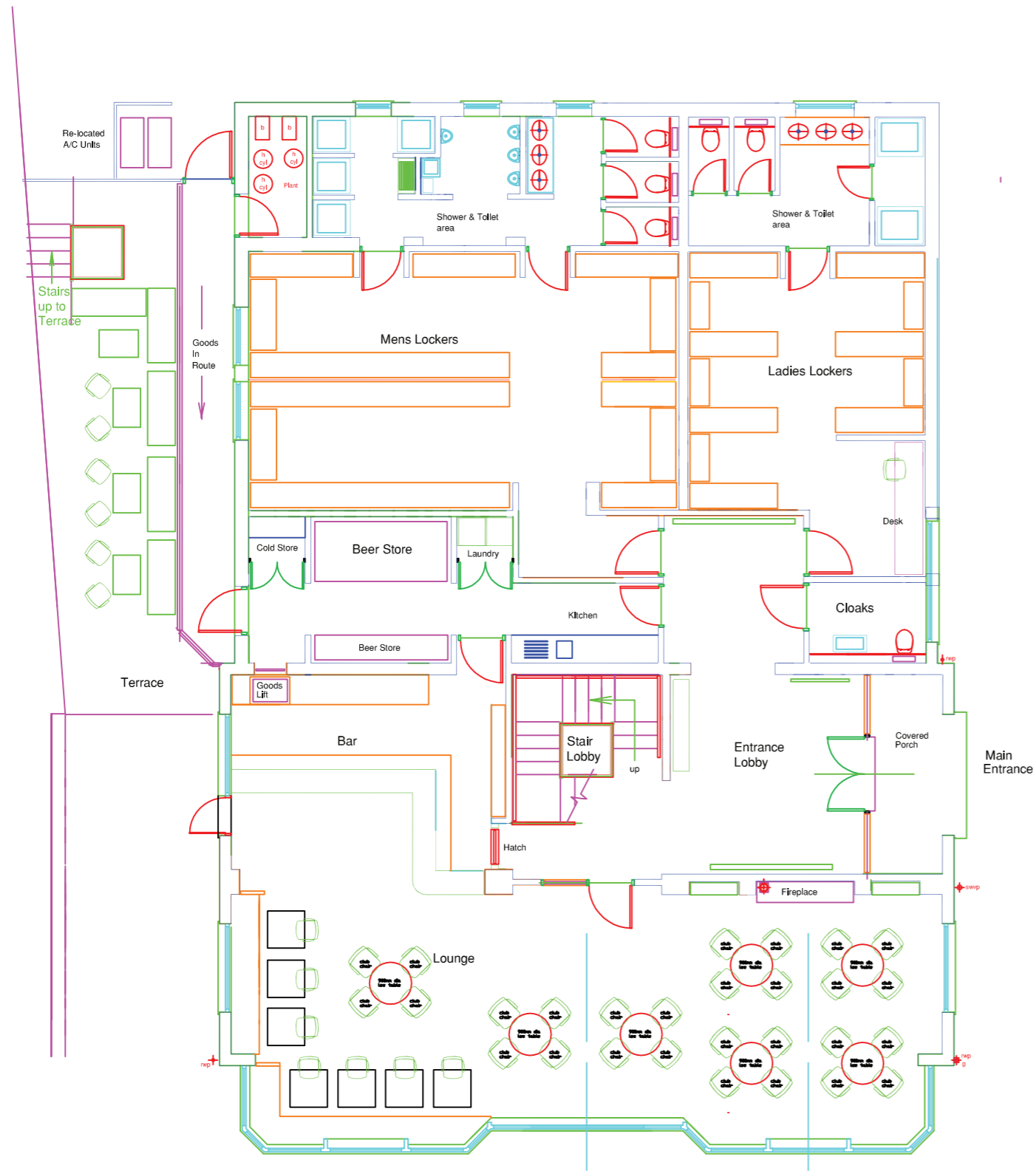
GOLF CLUBHOUSE GROUND FLOOR CONCEPT DESIGN
