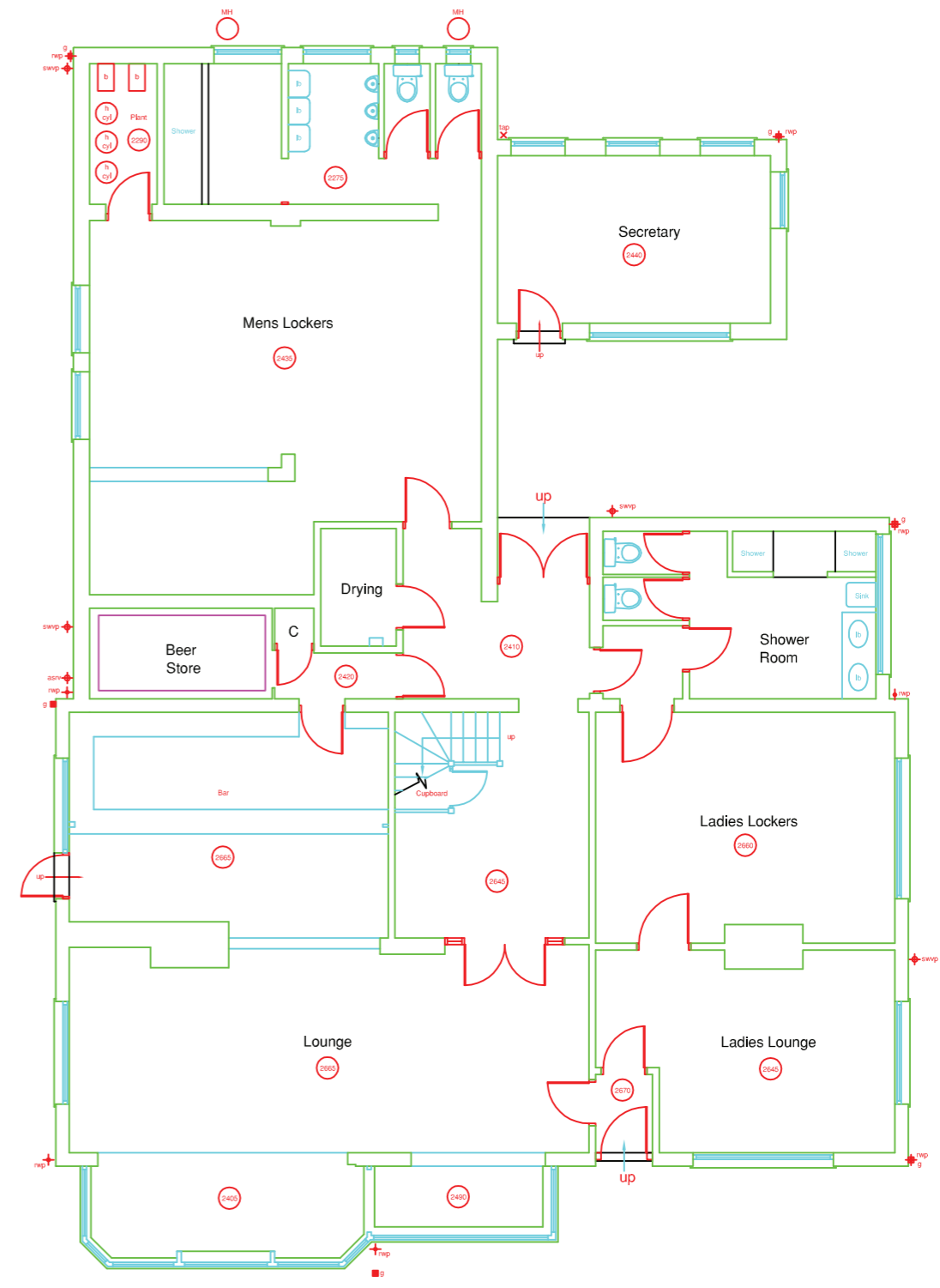
GOLF CLUBHOUSE GROUND FLOOR EXISTING LAYOUT
